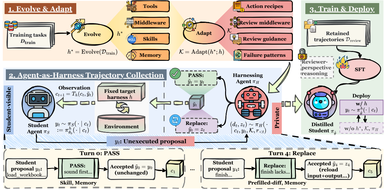
Figure 1: Overview of HARNES-ZERO. (1) Evolve and adapt. We evolve a student-side harness h^* (tools, middleware, skills, memory) on training tasks, and adapt it into a private reference harness \mathcal{K} (action recipes, review middleware, review guidance, failure patterns) relative to the fixed target harness h . (2) Agent-as-harness trajectory collection. The student \pi_S runs under h and proposes response y_t at each turn. The harnessing agent \pi_H reviews it using \mathcal{K} and either passes it unchanged or replaces it ( \tilde{y}_t ). Only \tilde{y}_t is executed through h and enters the student-visible context, while the review remains private. (3) Train and deploy. We apply SFT to the reviewed trajectories \mathcal{D}_{\text{review}} , masking any inadvertent reviewer-perspective reasoning from the loss. The distilled student is deployed under h alone, without h^* , \mathcal{K} , or \pi_H .
